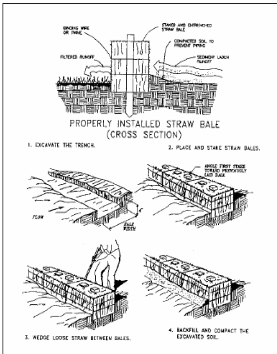
Figure 1. Properly installed straw bale and construction of straw bale barrier.
