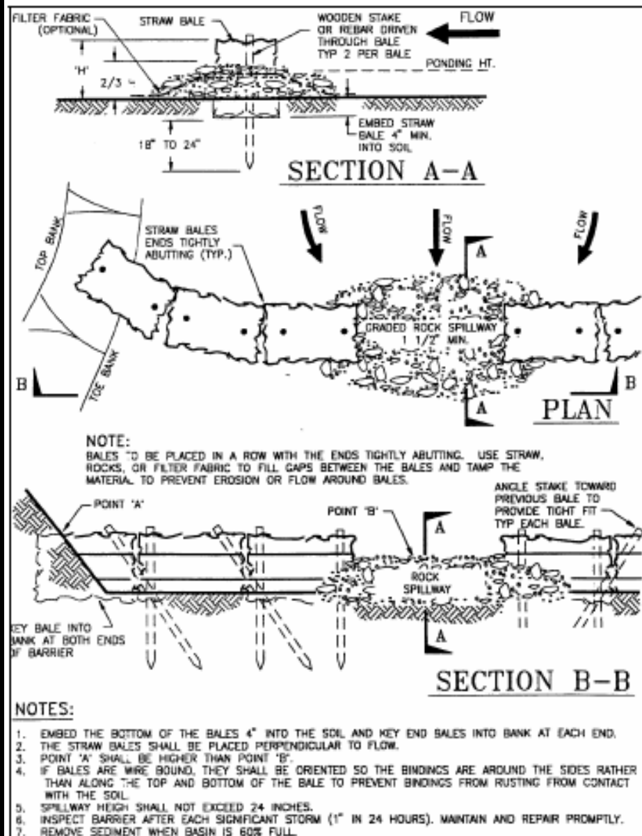
Figure 2. Semi-pervious straw bale sediment barrier, with sand and gravel spillway.
